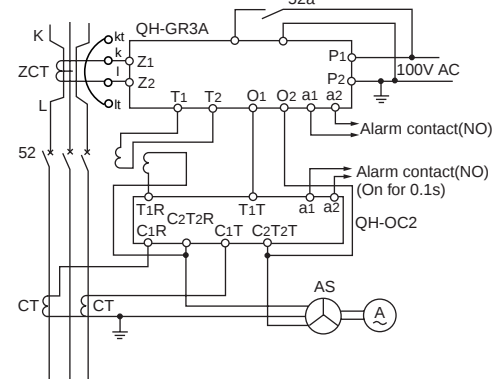
QH-GR3, current trip
