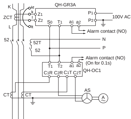
QH-GR3, shunt-trip
