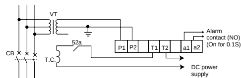
QH-OV1, QH-UV1
