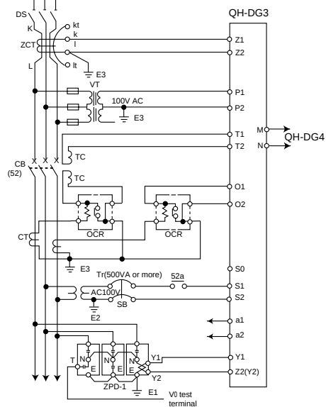
QH-DG3, current trip
