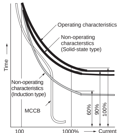
The inertia characteristics of Auto. V and induction type OCR
